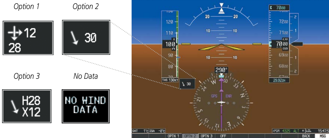
Figure 2-30 Wind Data
