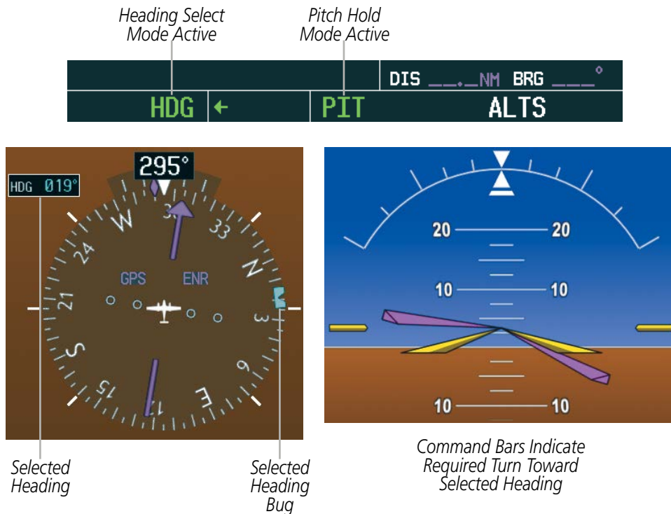
Figure 7-22 Heading Select Mode
