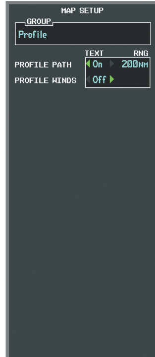
Figure 6-66 Navigation Map Page Setup Menu, Profile Group
