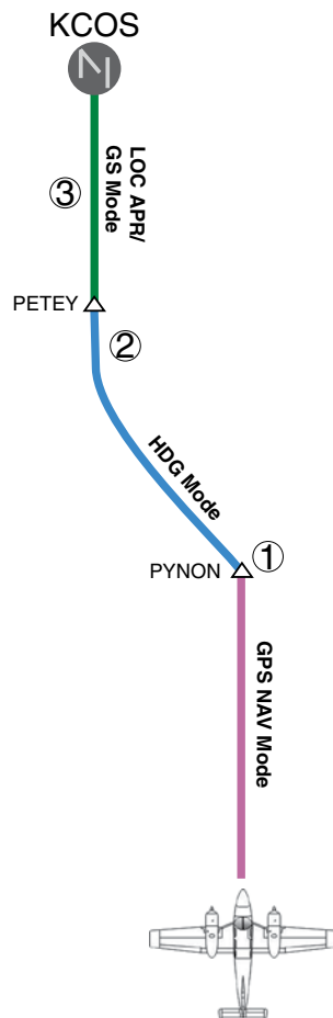
Figure 7-43 ILS Approach to KCOS
