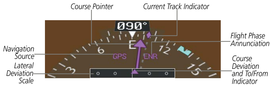
Figure 2-14 Arc HSI
