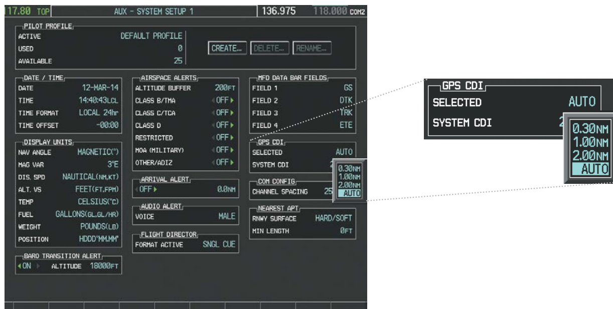
Figure 2-23 GPS CDI Setting (AUX - System Setup Page)
