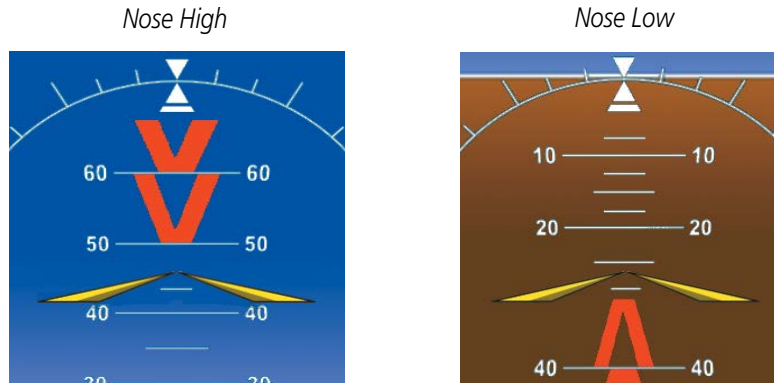
Figure 2-41 Pitch Attitude Warnings
