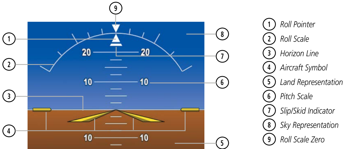
Figure 2-5 Attitude Indicator
