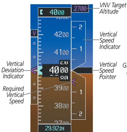
Figure 2-10 Vertical Speed and Deviation Indicator (VSI and VDI)
