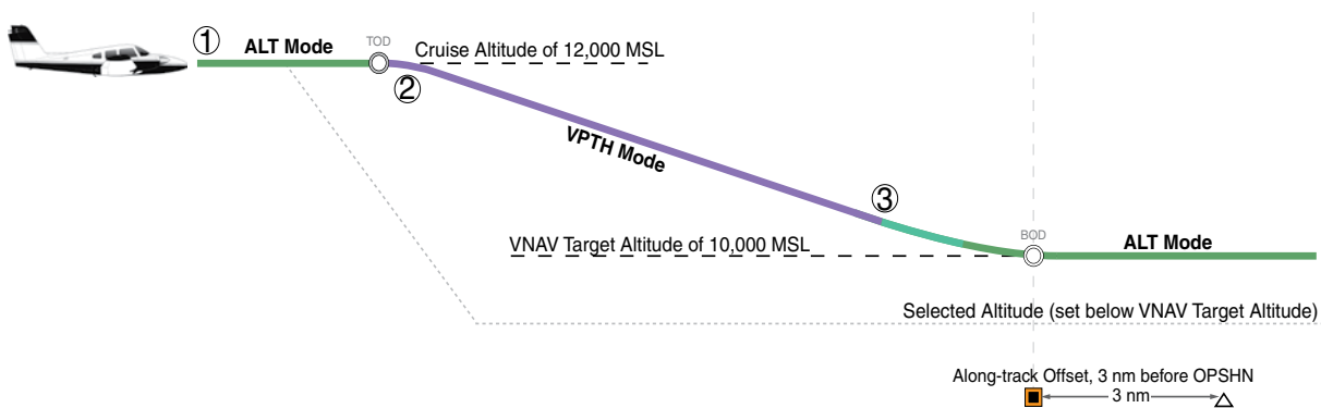
Figure 7-41 VPTH Descent
