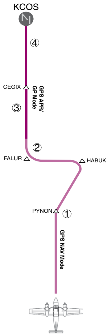
Figure 7-44 LPV Approach to KCOS
