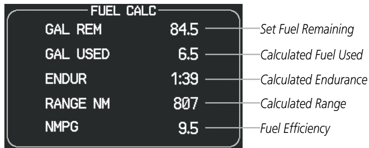
Figure 3-9 Fuel Calculations Group
