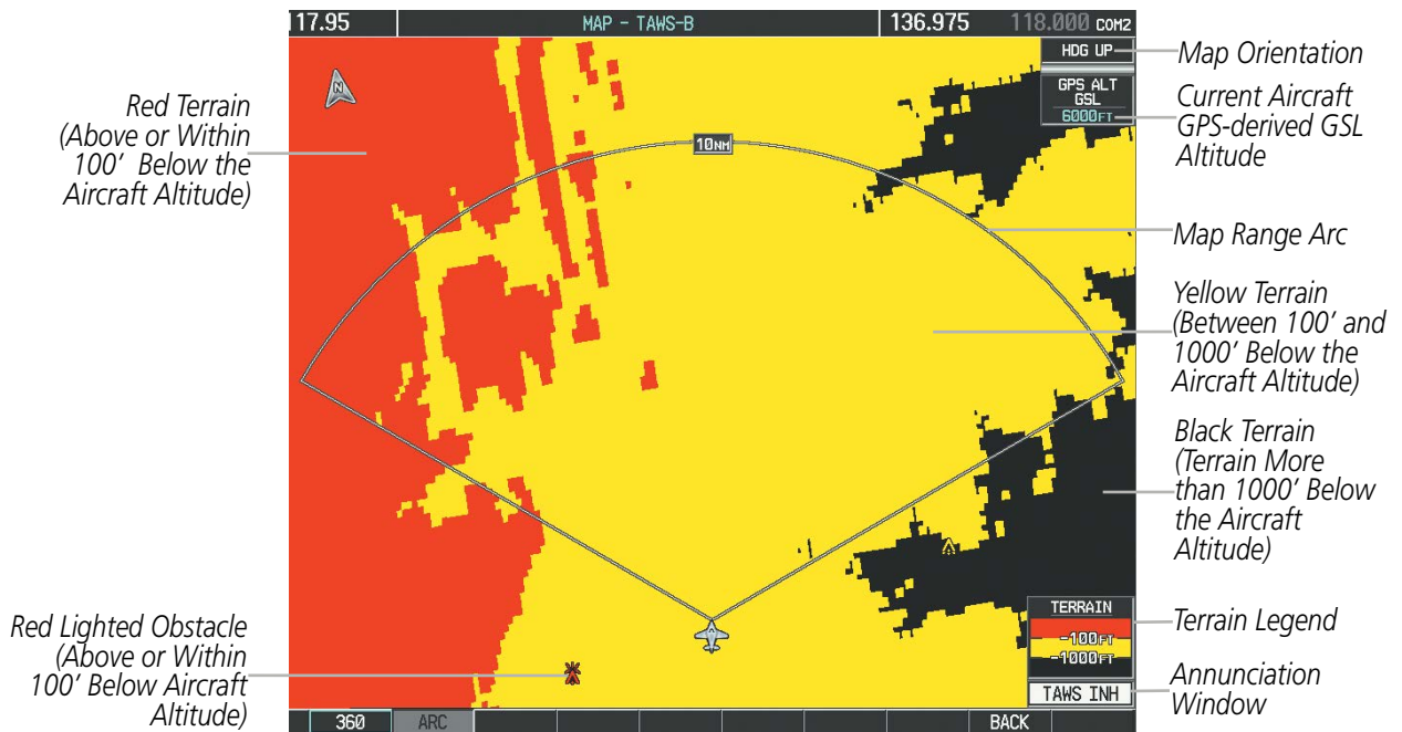
Figure 6-83 TAWS-B Page (ARC View)
