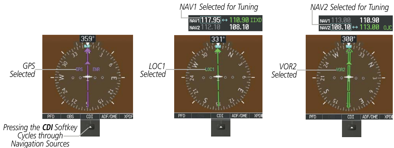
Figure 2-22 Selecting a Navigation Source
