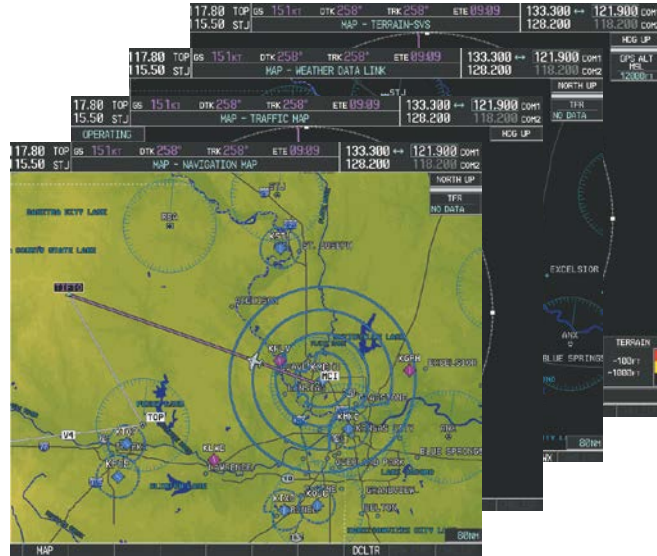
Figure 1-23 Map Pages
