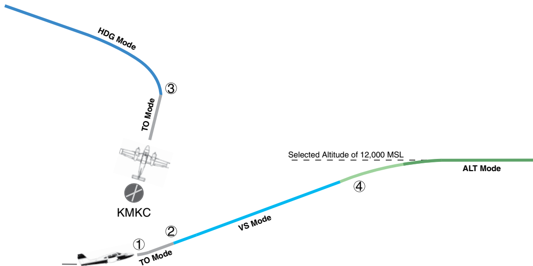
Figure 7-37 Departure
