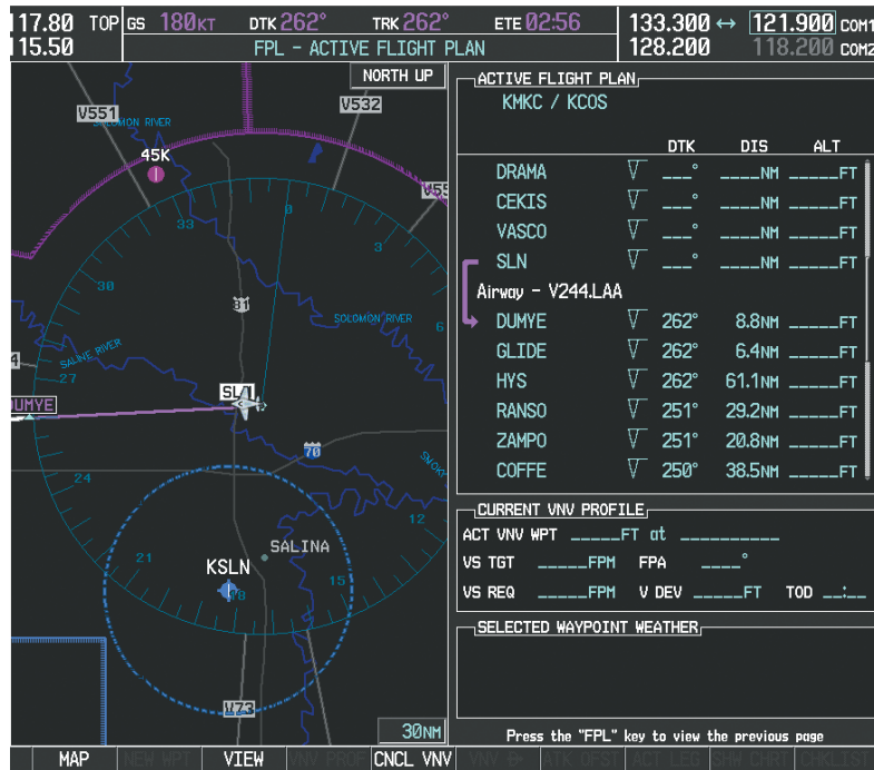
Figure 5-125 V244 Now Active Leg
