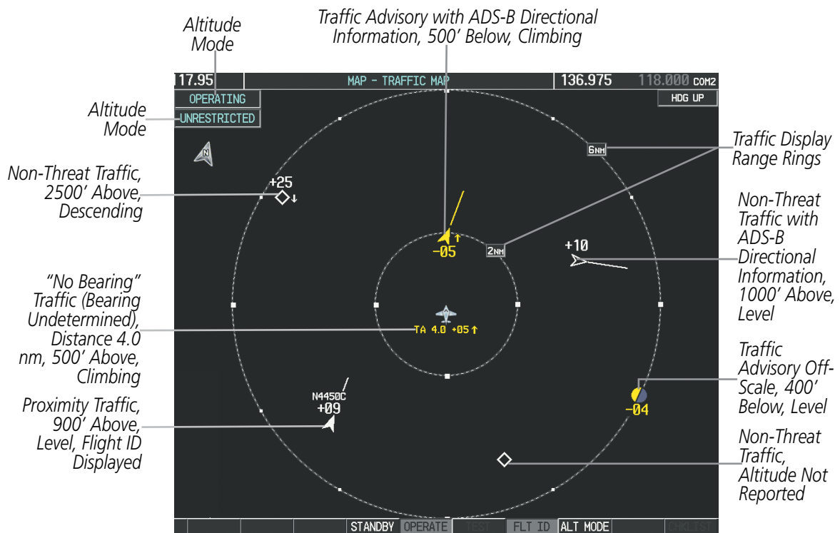
Figure 6-104 Traffic Map Page
