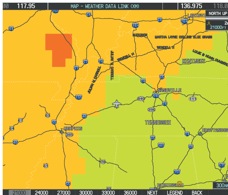
Figure 6-44 Turbulence Weather Product at 21,000 Feet
