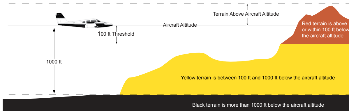
Figure 6-55 Terrain Altitude/Color Correlation for Terrain Proximity
