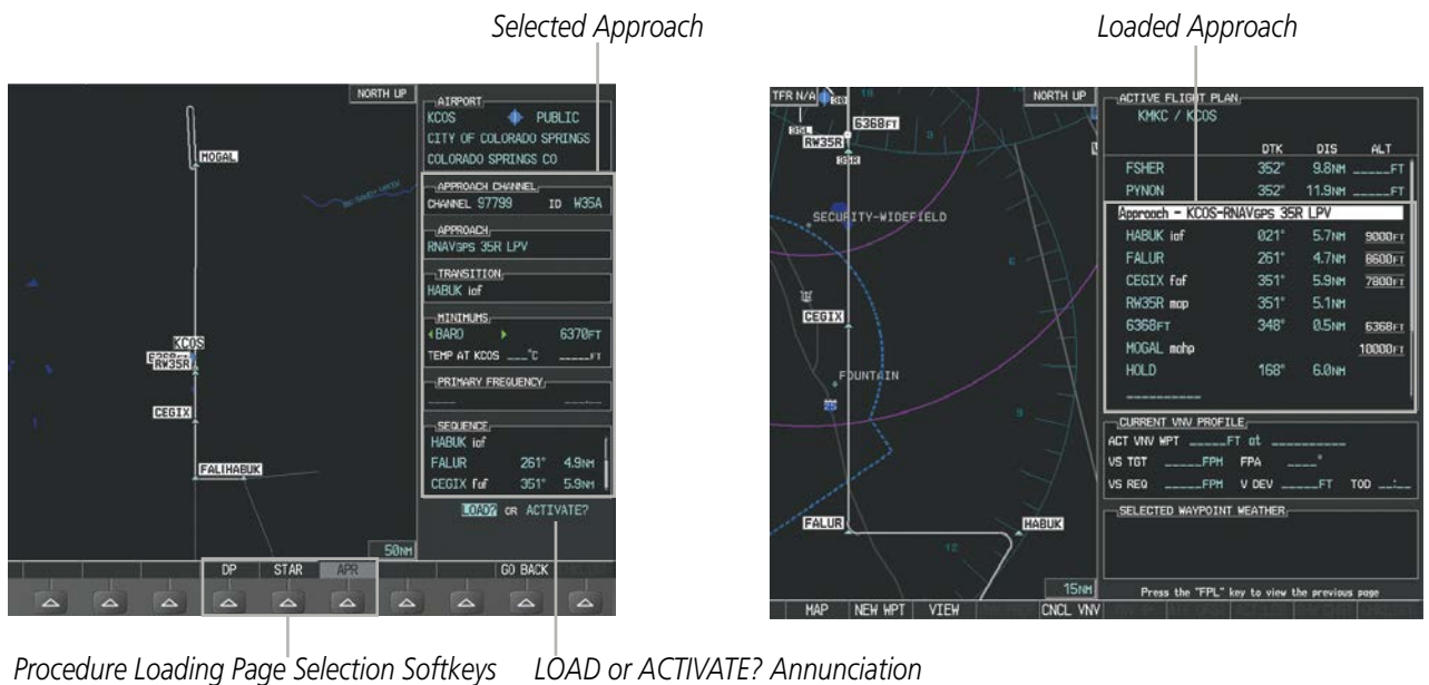
Figure 5-100 Approach Loading
