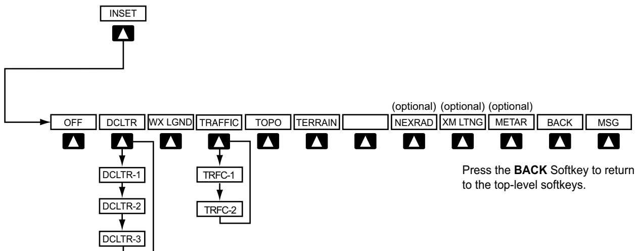
Figure 1-17 INSET Softkeys
