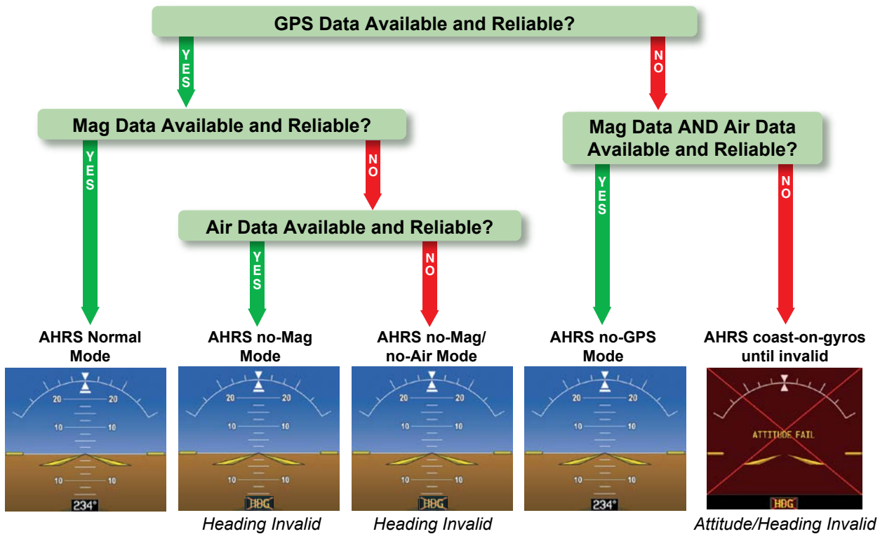
Figure 1-9 AHRS Operation
