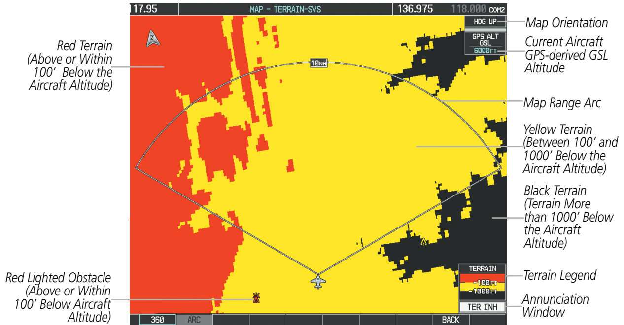
Figure 6-72 Terrain-SVS Page (ARC View)
