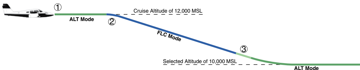
Figure 7-40 FLC Descent
