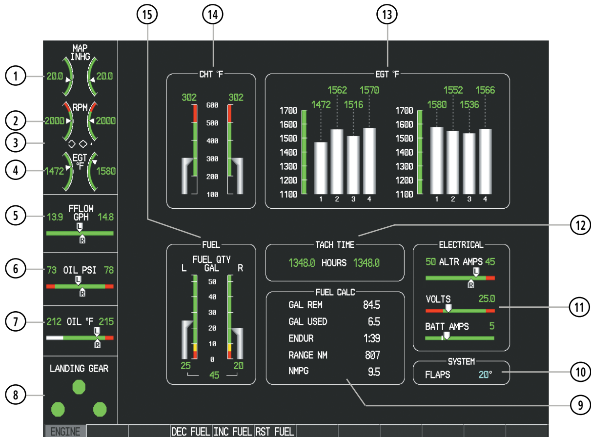
Figure 3-5 Engine Page
