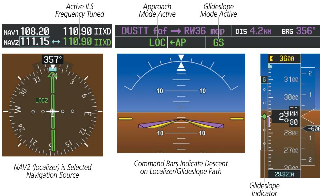
Figure 7-18 Glideslope Mode
