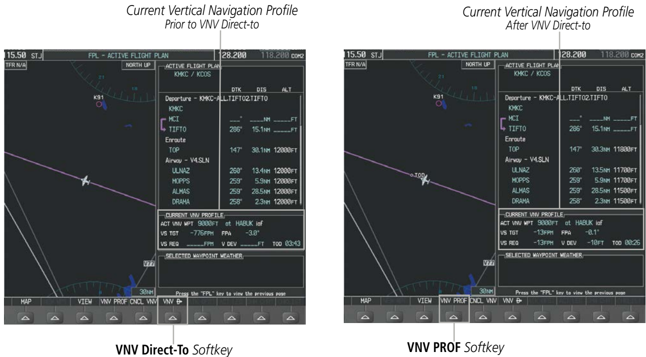
Figure 5-93 Vertical Navigation Direct-To
