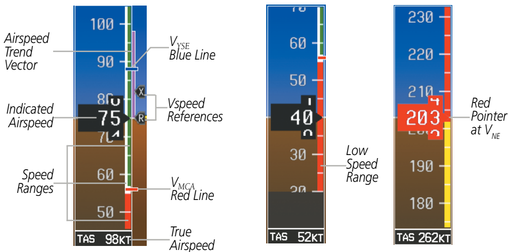
Figure 2-3 Airspeed Indicator Ranges
