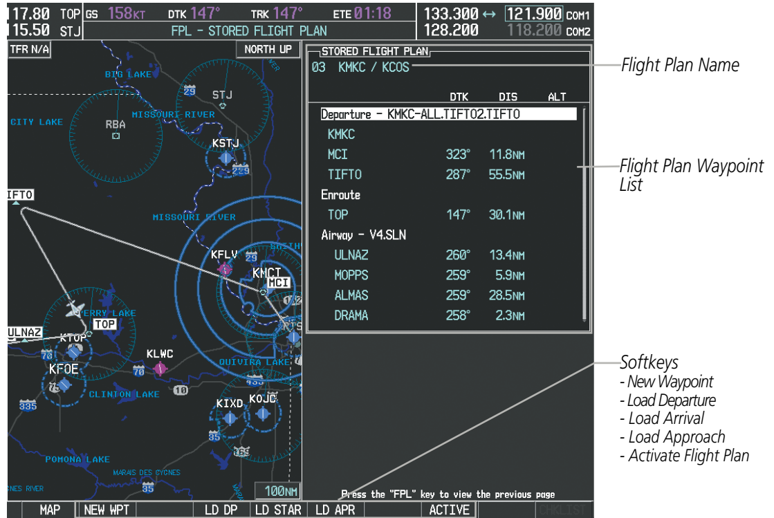
Figure 5-67 Stored Flight Plan Page
