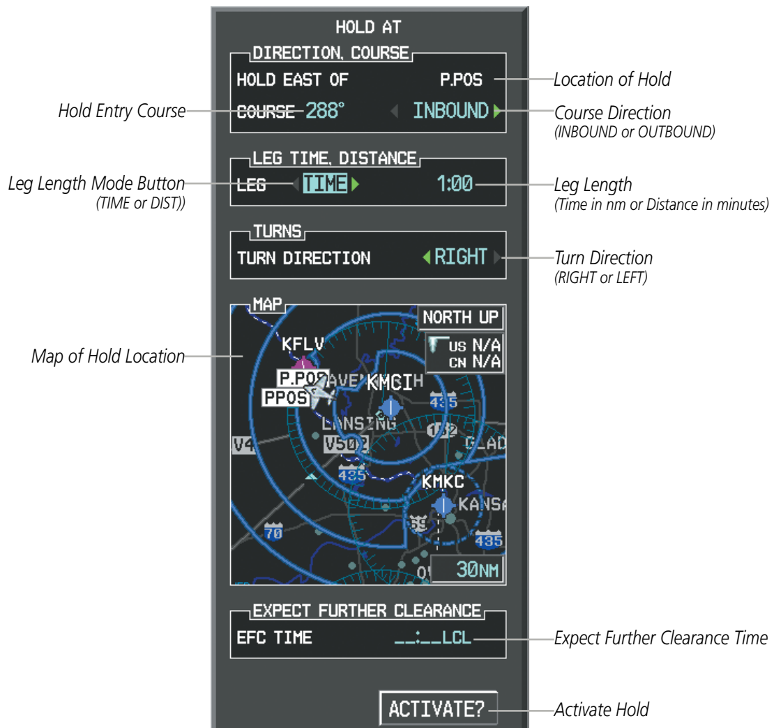
Figure 5-90 Creating a User Defined Holding Pattern at the Aircraft Present Position
