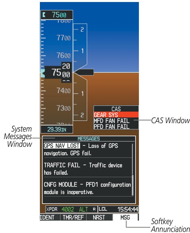
Figure 2-32 G1000 Alerting System
