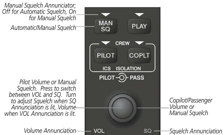
Figure 4-43 Volume/Squelch Control
