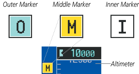
Figure 2-33 Marker Beacon Annunciations
