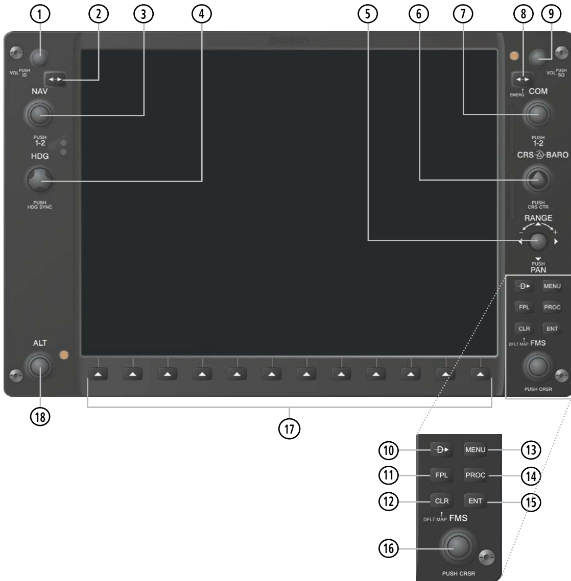
Figure 1-12 PFD/MFD Controls
