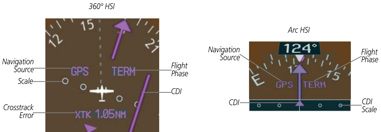
Figure 2-20 Course Deviation Indicator
