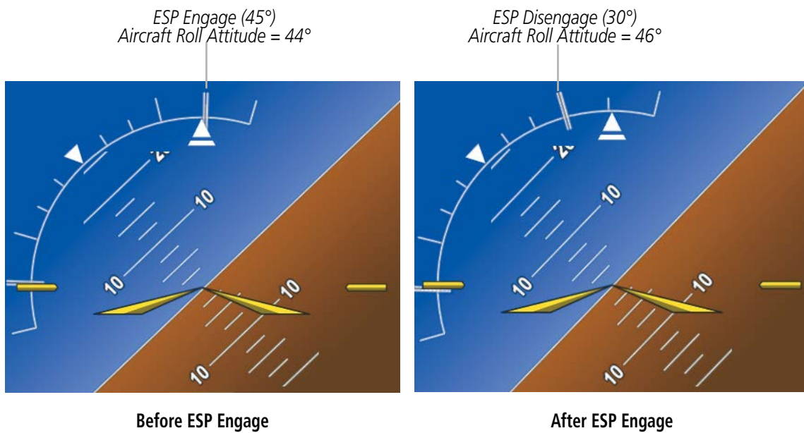
Figure 8-84 Roll Increasing to ESP Engagement
