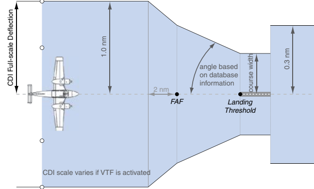
Figure 2-26 Typical LNAV/VNAV, LPV and LP Approach CDI Scaling
