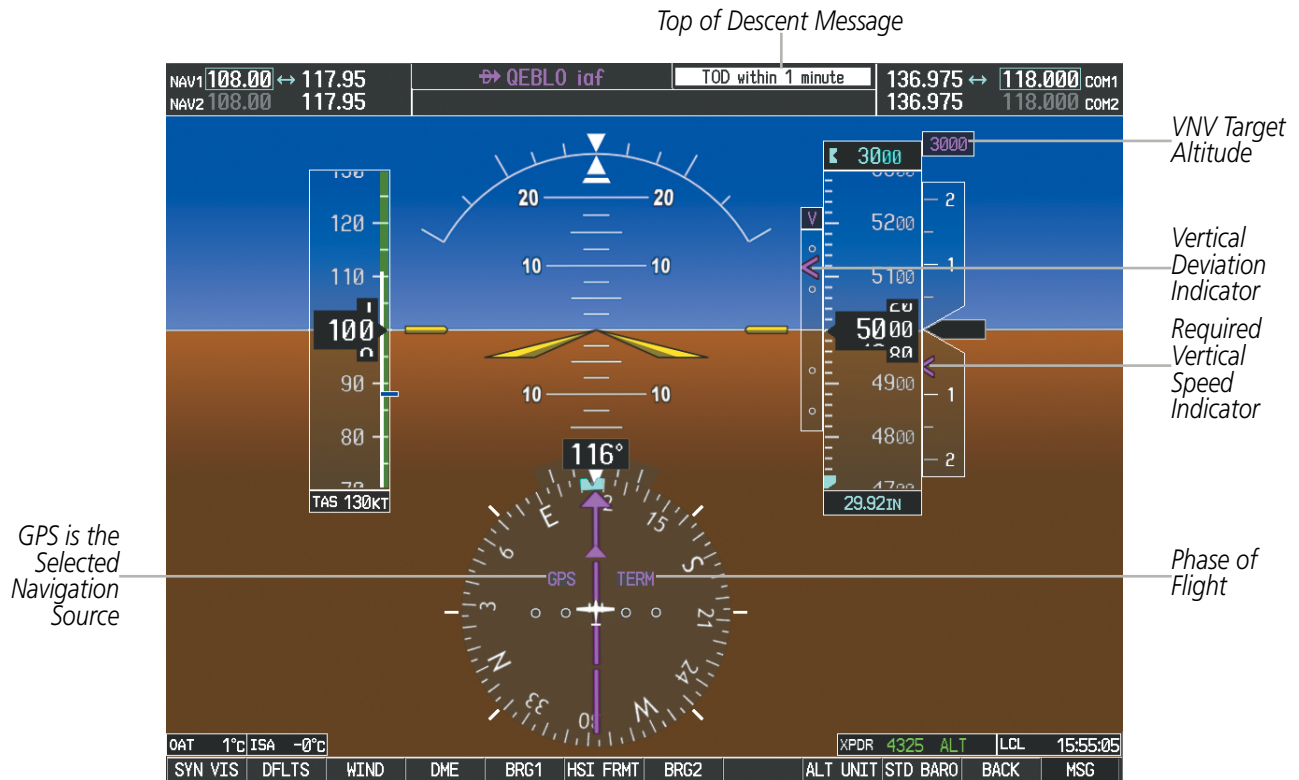
Figure 2-31 Vertical Navigation Indications (PFD)
