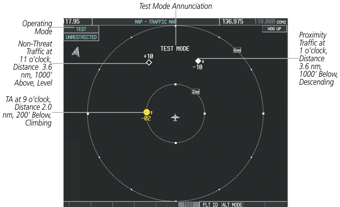
Figure 6-103 System Test in Progress with Test Pattern
