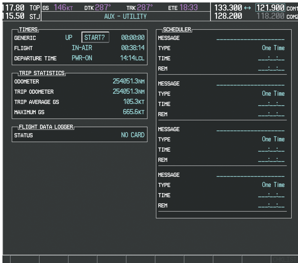
Figure 1-33 Utility Page
