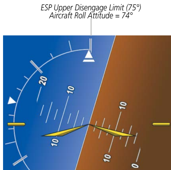
Figure 8-86 Roll Attitude Autopilot Engagement Limit (ESP Engaged)
