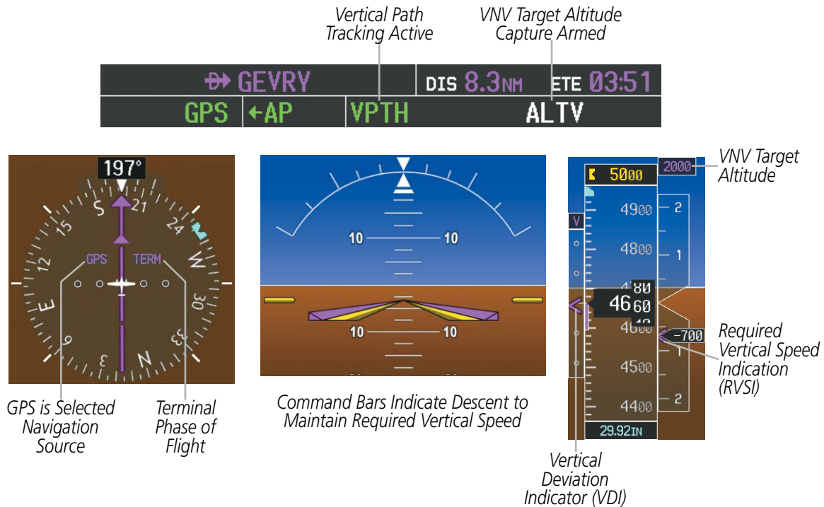
Figure 7-12 Vertical Path Tracking Mode
