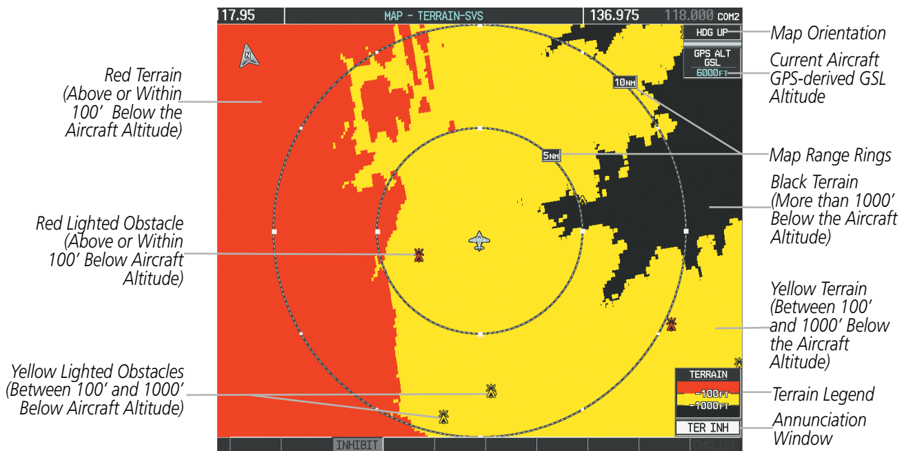
Figure 6-71 Terrain-SVS Page
