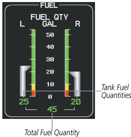
Figure 3-13 Fuel Display
