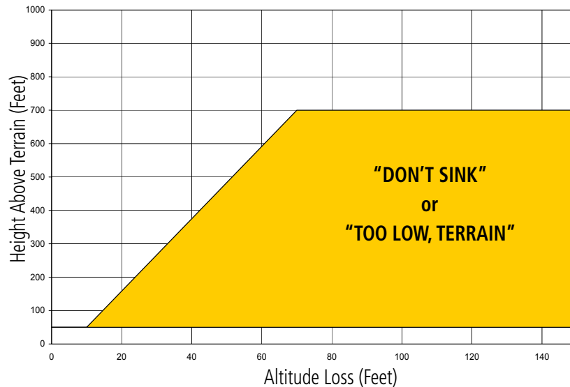
Figure 6-90 Negative Climb Rate (NCR) Altitude Loss
