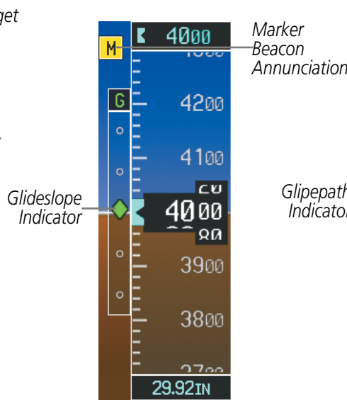
Figure 2-11 Glideslope Indicator
