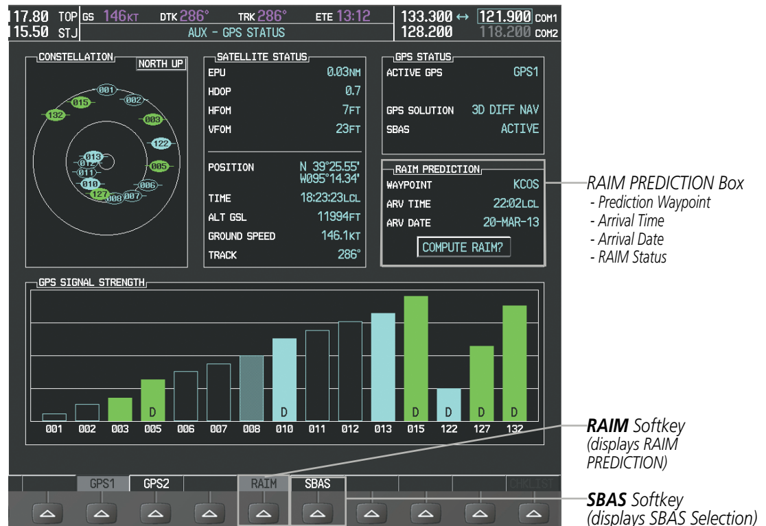
Figure 5-109 RAIM Prediction
