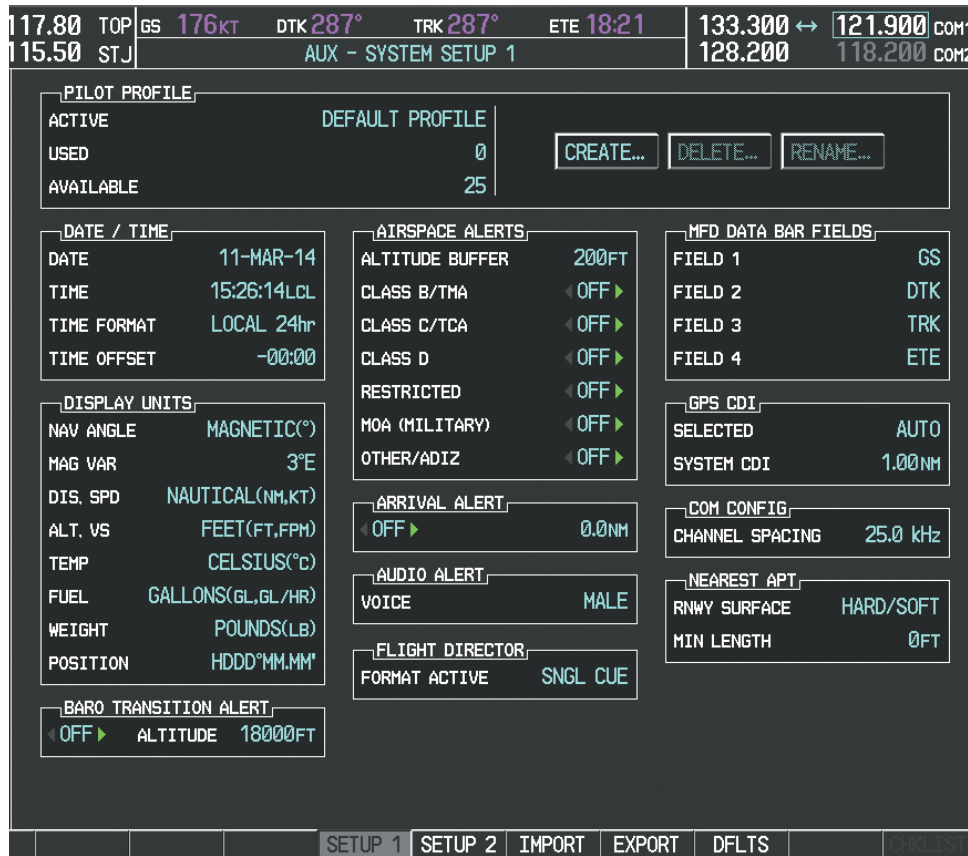
Figure 1-29 System Setup 1 Page
