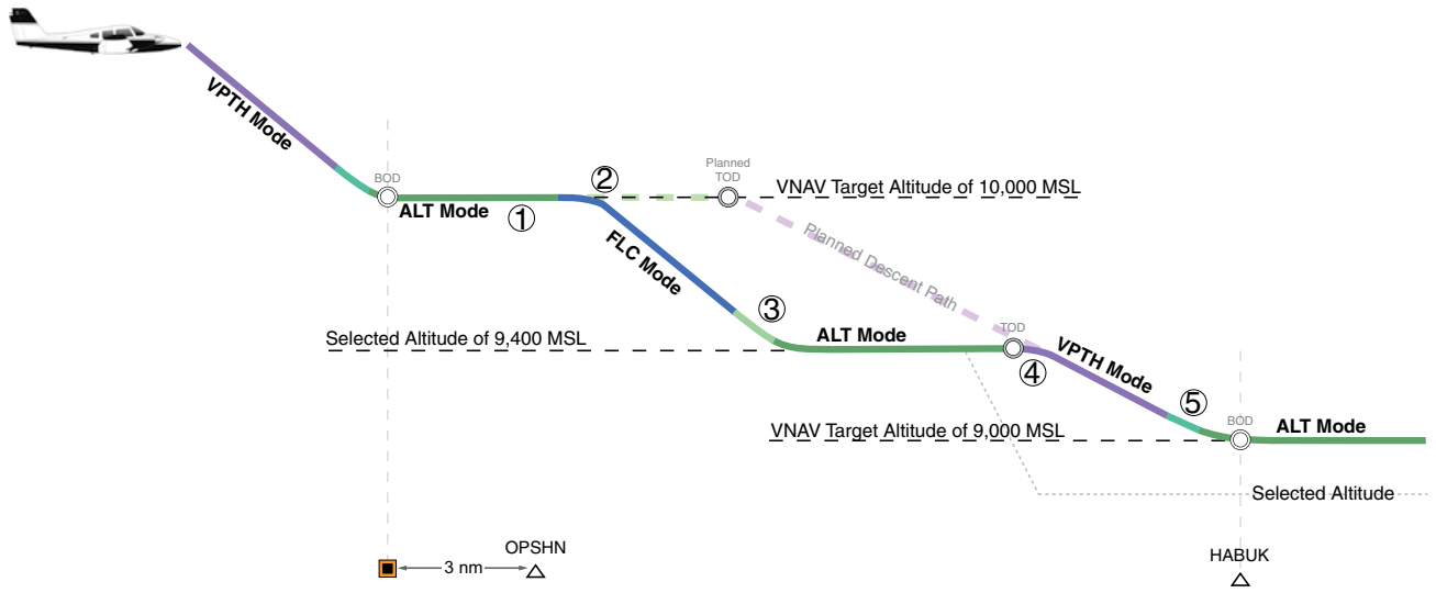
Figure 7-42 Non-path Descent
