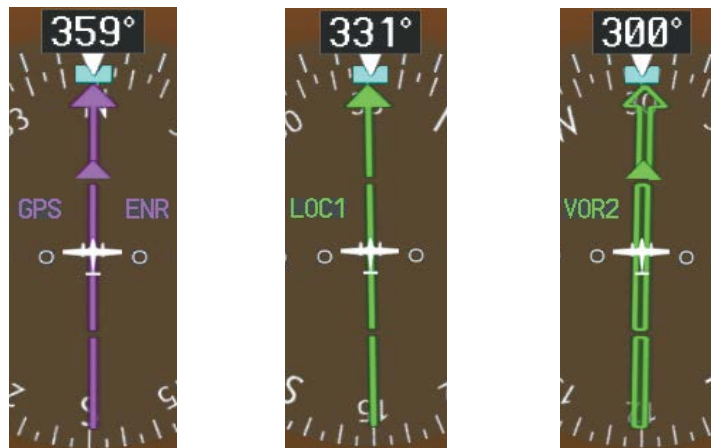
Figure 2-21 Navigation Sources
