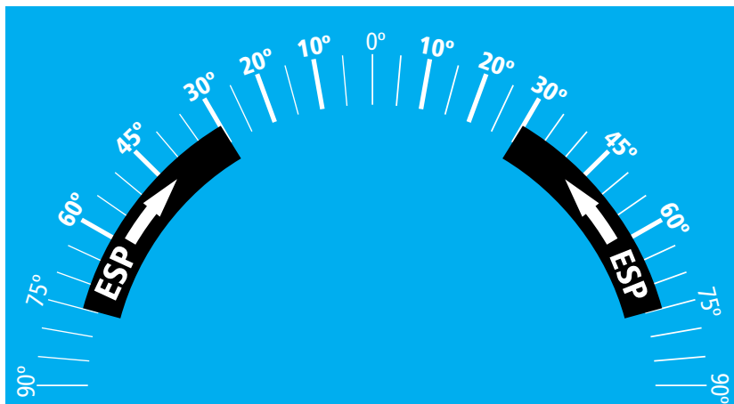
Figure 8-85 ESP Roll Operating Range When Engaged (Force Increases as Roll Increases & Decreases as Roll Decreases)
