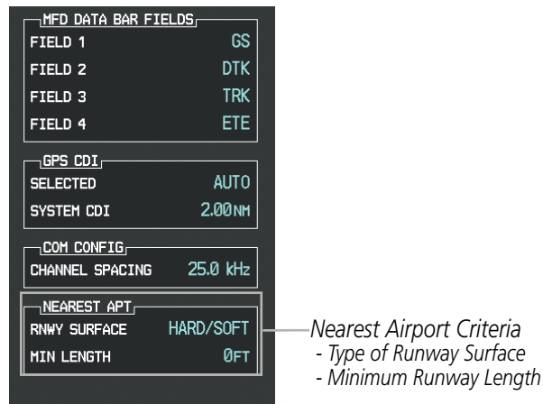
Figure 5-38 System Setup Page - Nearest Airport Selection Criteria
