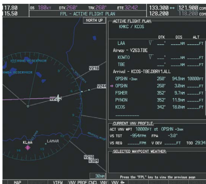
Figure 5-130 Direct-to Active
