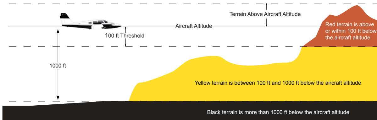
Figure 6-62 Terrain Altitude/Color Correlation for Profile View Terrain
