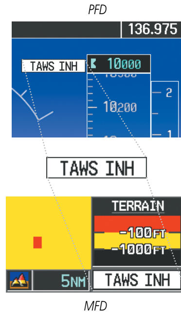
Figure 6-89 TAWS-B Alerting Inhibited Annunciation
