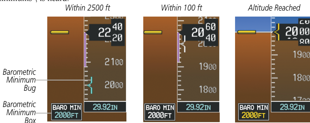
Figure 2-38 Barometric MDA/DH Alerting Visual Annunciations
