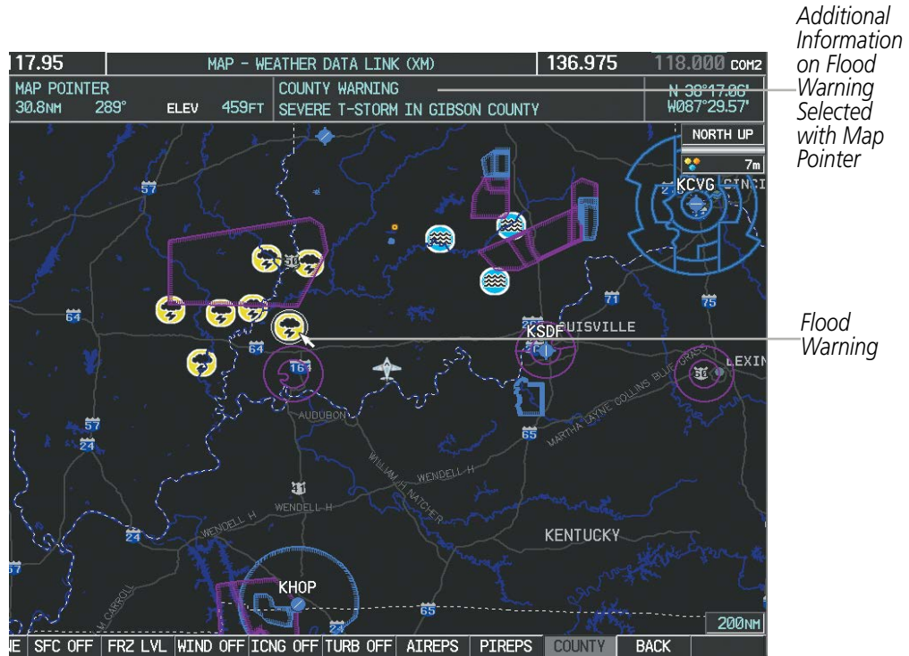
Figure 6-38 County Flood Warning
