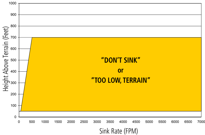
Figure 6-91 Negative Climb Rate (NCR) Sink Rate
