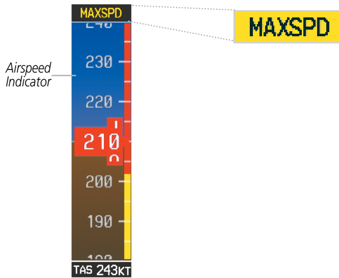
Figure 7-47 Overspeed Annunciation
