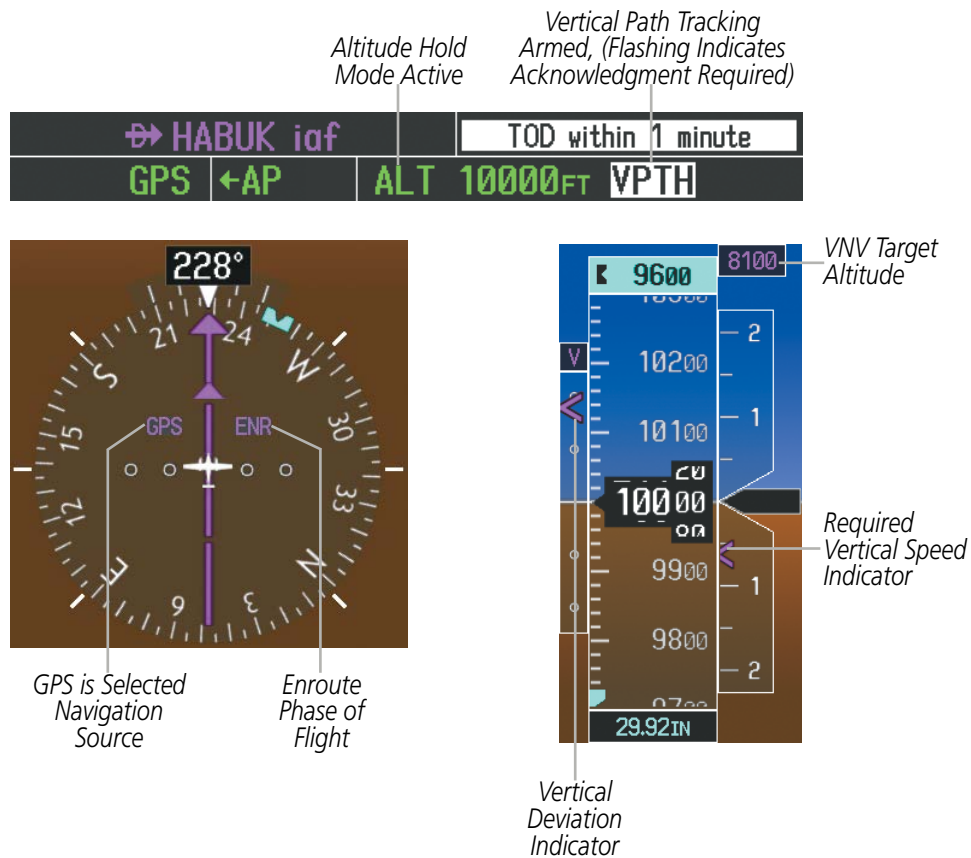
Figure 7-11 Vertical Path Capture
