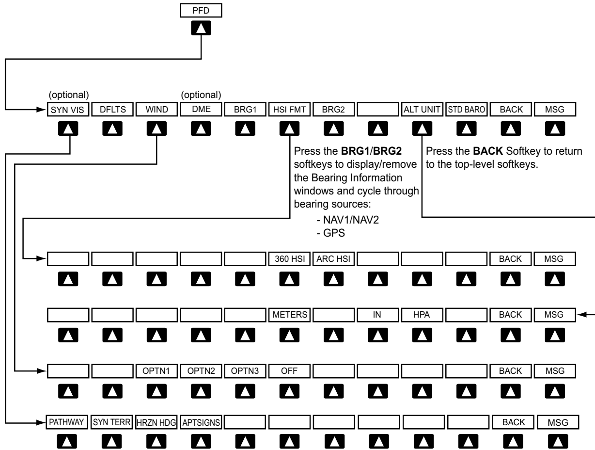
Figure 1-18 PFD Configuration Softkeys
