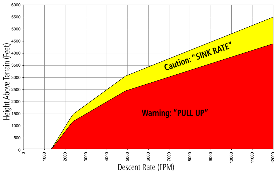
Figure 6-86 Excessive Descent Rate Alert Criteria
