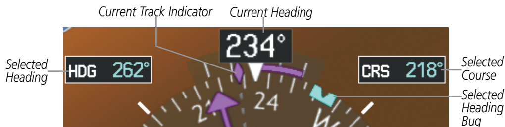
Figure 2-15 Heading and Course Indications
