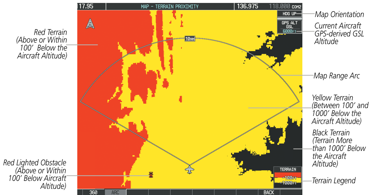
Figure 6-61 Terrain Proximity Page (ARC View)
