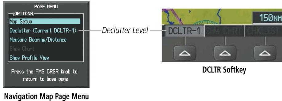
Figure 5-21 Navigation Map - Declutter Level Indications
