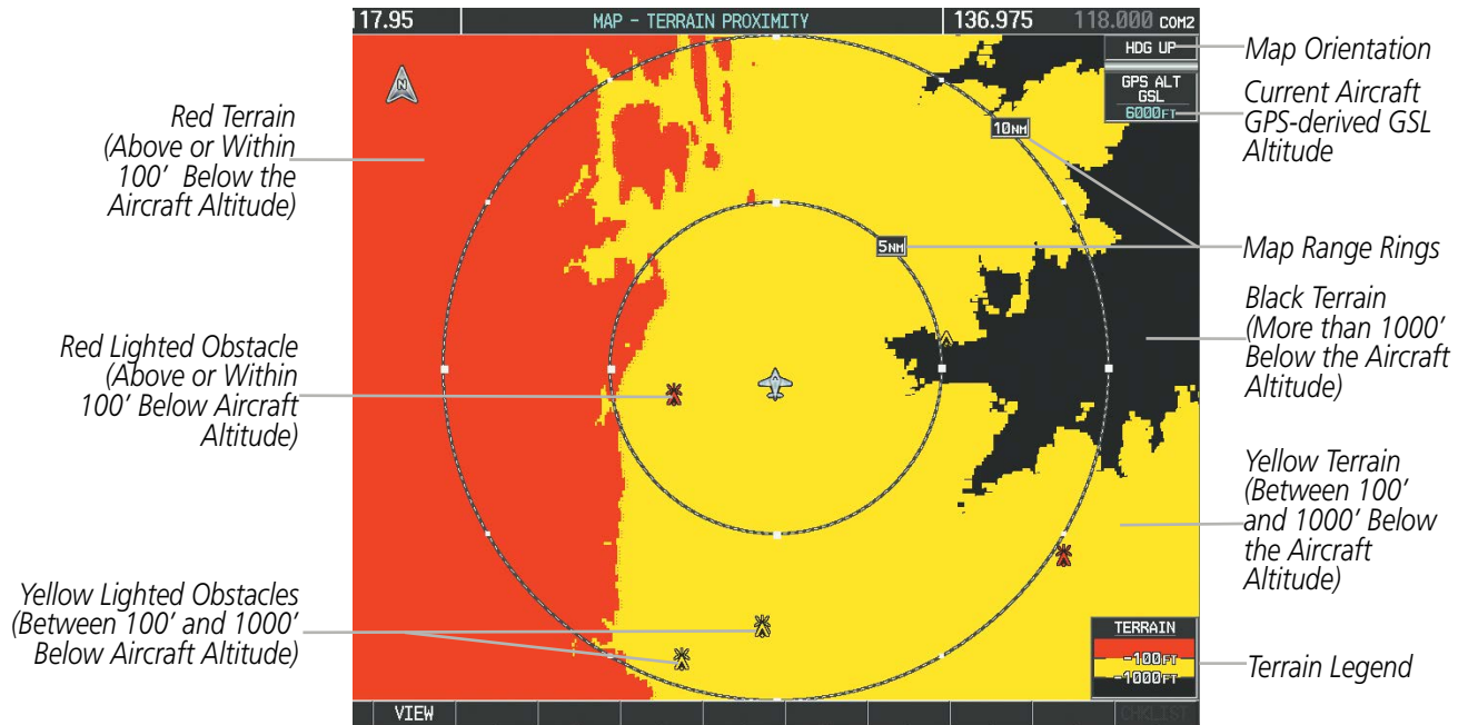
Figure 6-60 Terrain Proximity Page
