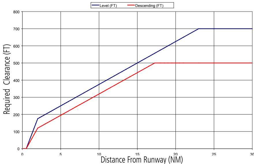
Figure 6-75 FLTA Alert Minimum Terrain and Obstacle Clearance Values
