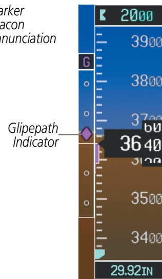
Figure 2-12 Glidepath Indicator
