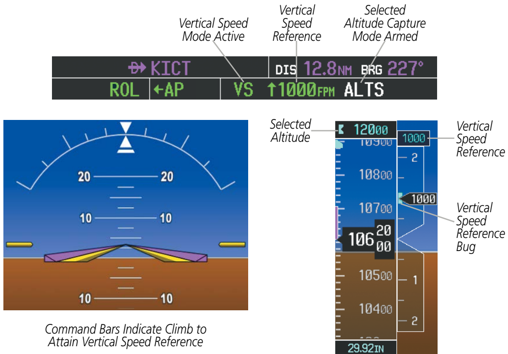
Figure 7-8 Vertical Speed Hold Mode
