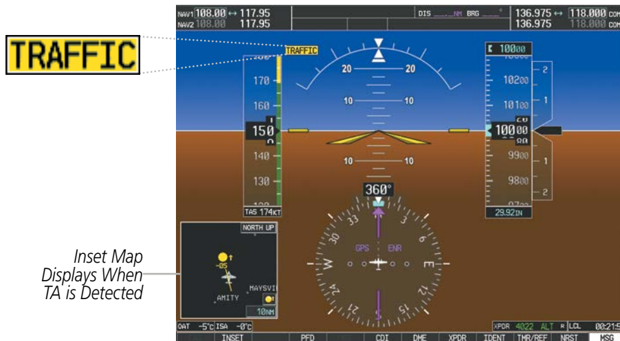
Figure 6-98 Traffic Annunciation (PFD)
