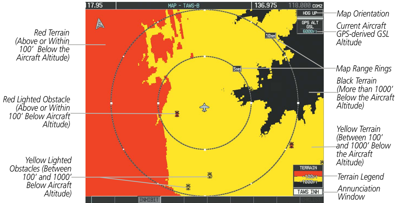
Figure 6-82 TAWS-B Page
