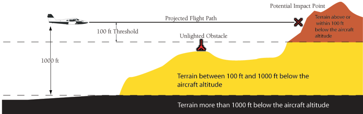
Figure 6-77 Terrain Altitude/Color Correlation for TAWS
