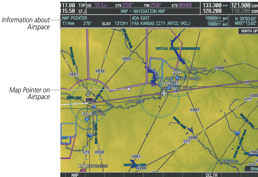
Figure 5-10 Navigation Map - Map Pointer on Airspace
