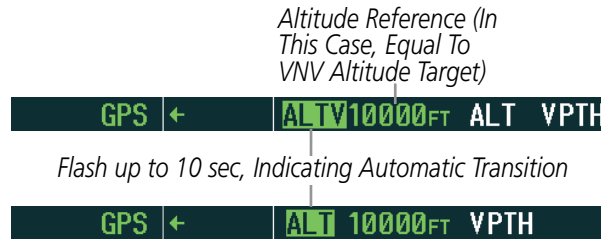
Figure 7-14 VNV Altitude Capture
