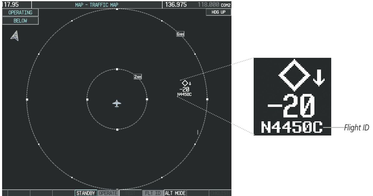
Figure 6-105 Traffic Map Page with Flight ID Enabled
