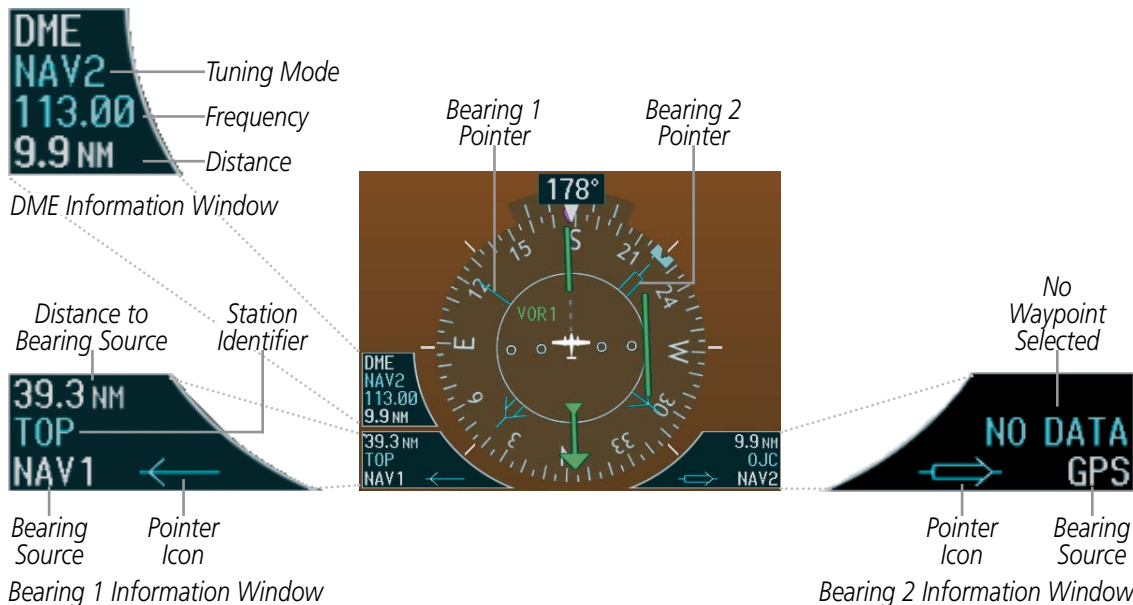
Figure 2-19 HSI with Bearing and DME Information
