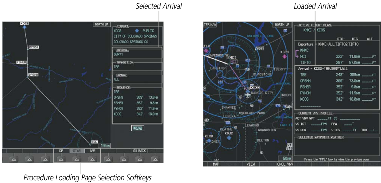
Figure 5-98 Arrival Loading
