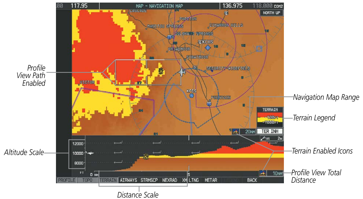
Figure 6-63 Navigation Map Page with Profile View Terrain and Topographic Data Enabled
