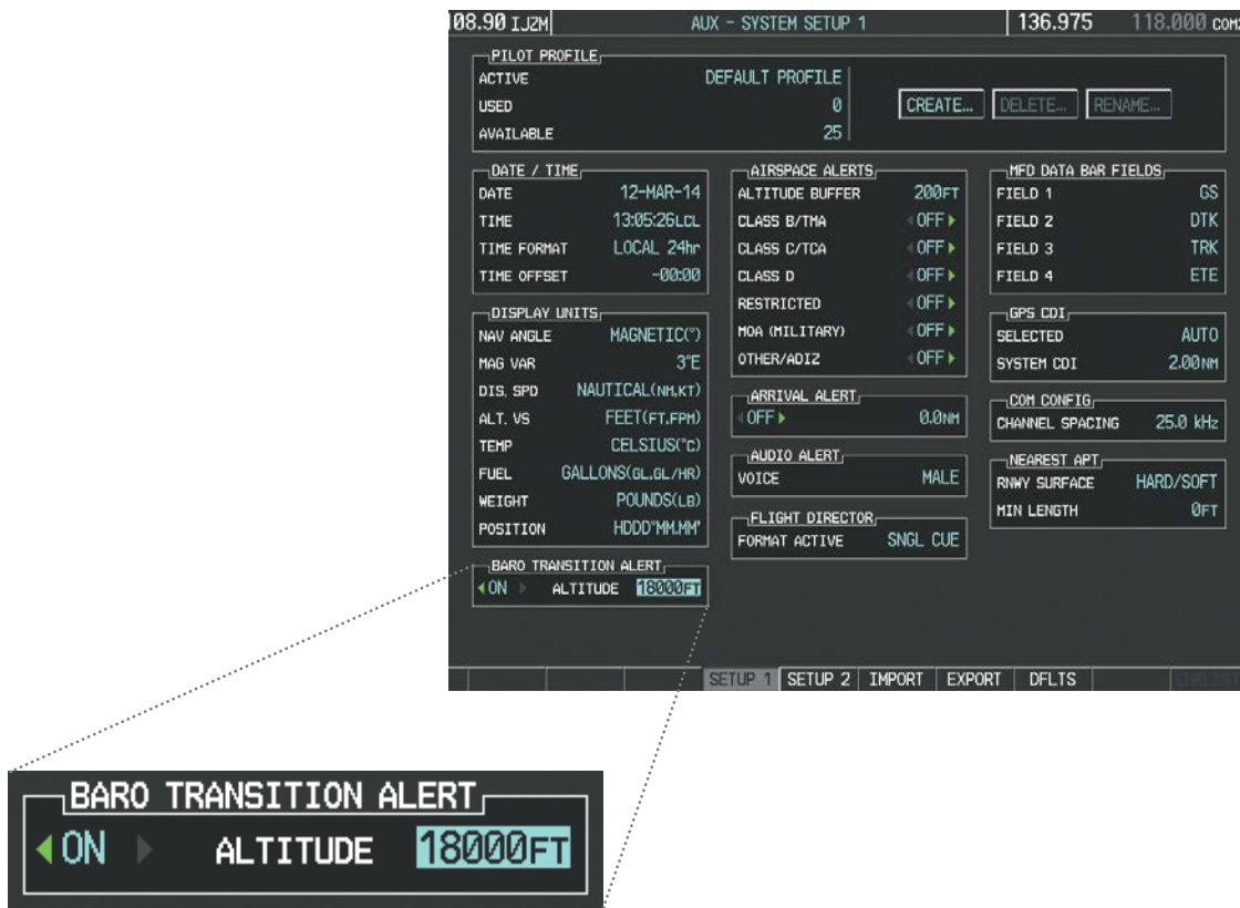
Figure 2-9 Baro Transition Alert (AUX - System Setup Page)
