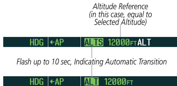
Figure 7-6 Automatic Mode Transitions During Altitude Capture
