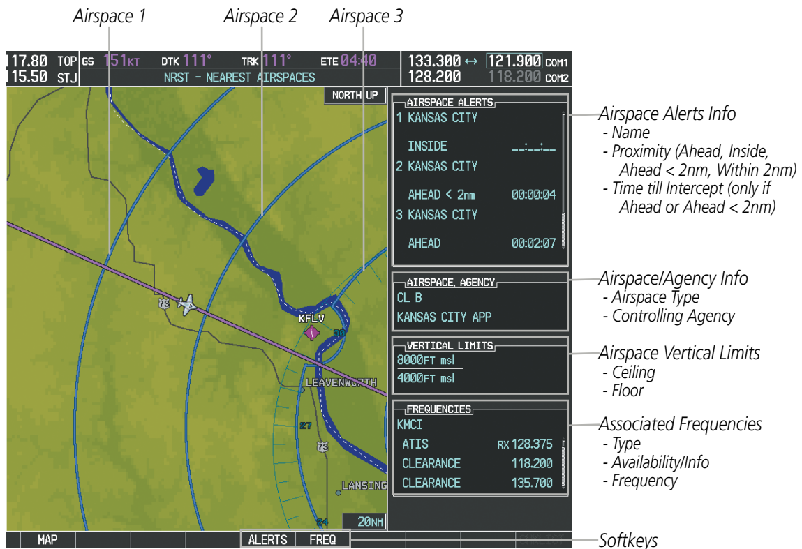
Figure 5-50 Nearest Airspaces Page
