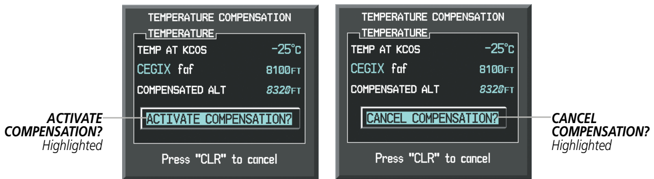
Figure 5-102 Activating/Canceling Temperature Compensation
