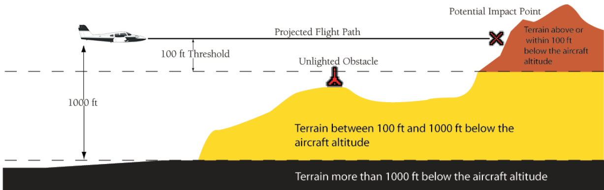
Figure 6-67 Terrain Altitude/Color Correlation for Terrain-SVS
