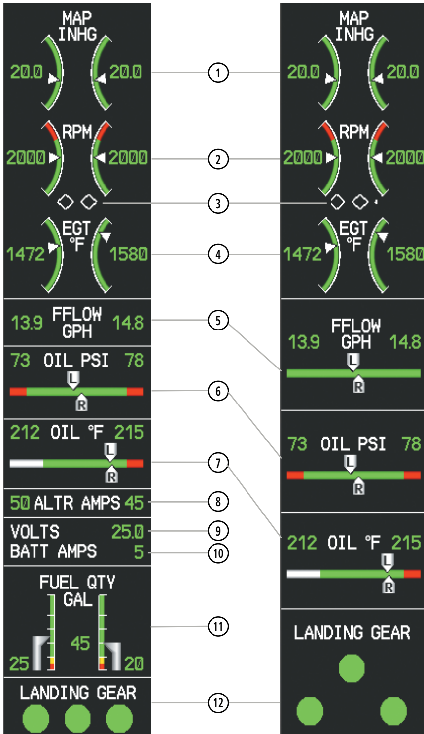
Figure 3-2 Engine Display
