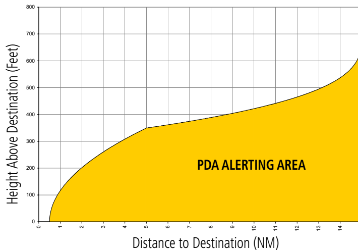
Figure 6-88 PDA Alerting Threshold
