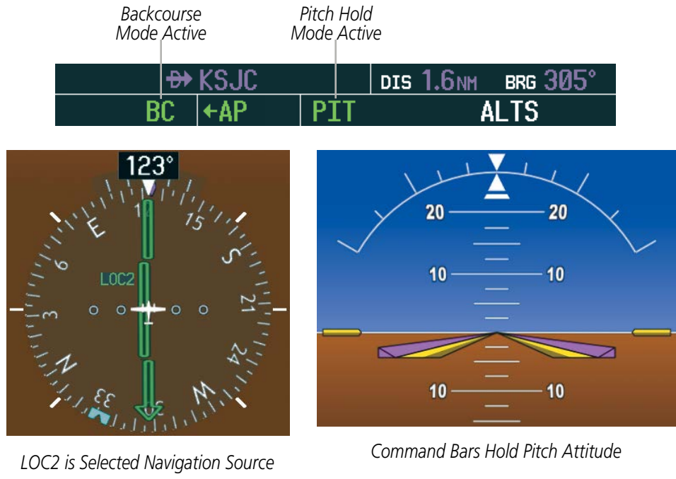
Figure 7-25 Backcourse Mode
