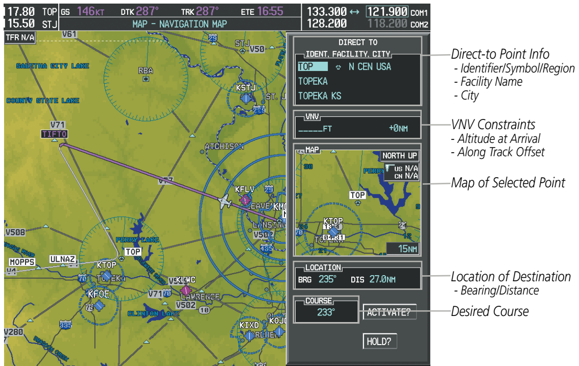
Figure 5-51 Direct-to Window - MFD
