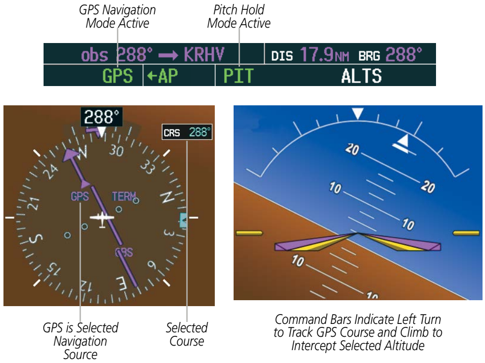
Figure 7-24 Navigation Mode
