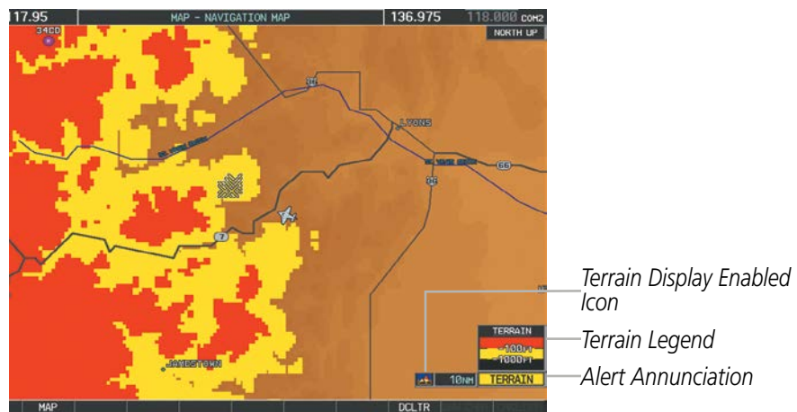
Figure 6-74 Navigation Map Page (After Terrain-SVS Pop-up Alert Acknowledgment)
