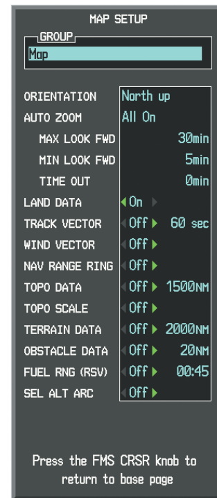
Figure 6-58 Navigation Map Page Setup Menu, Map Group
