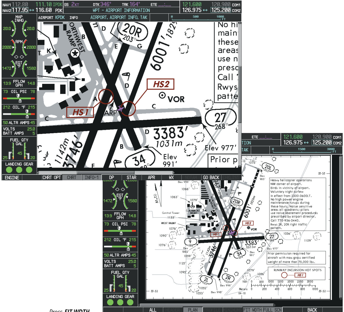
Figure 8-40 Airport Information Page, FIT WDTN Softkey Selected
