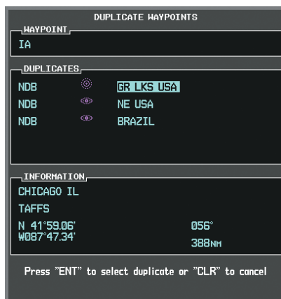
Figure 5-63 Duplicate Waypoints Window
