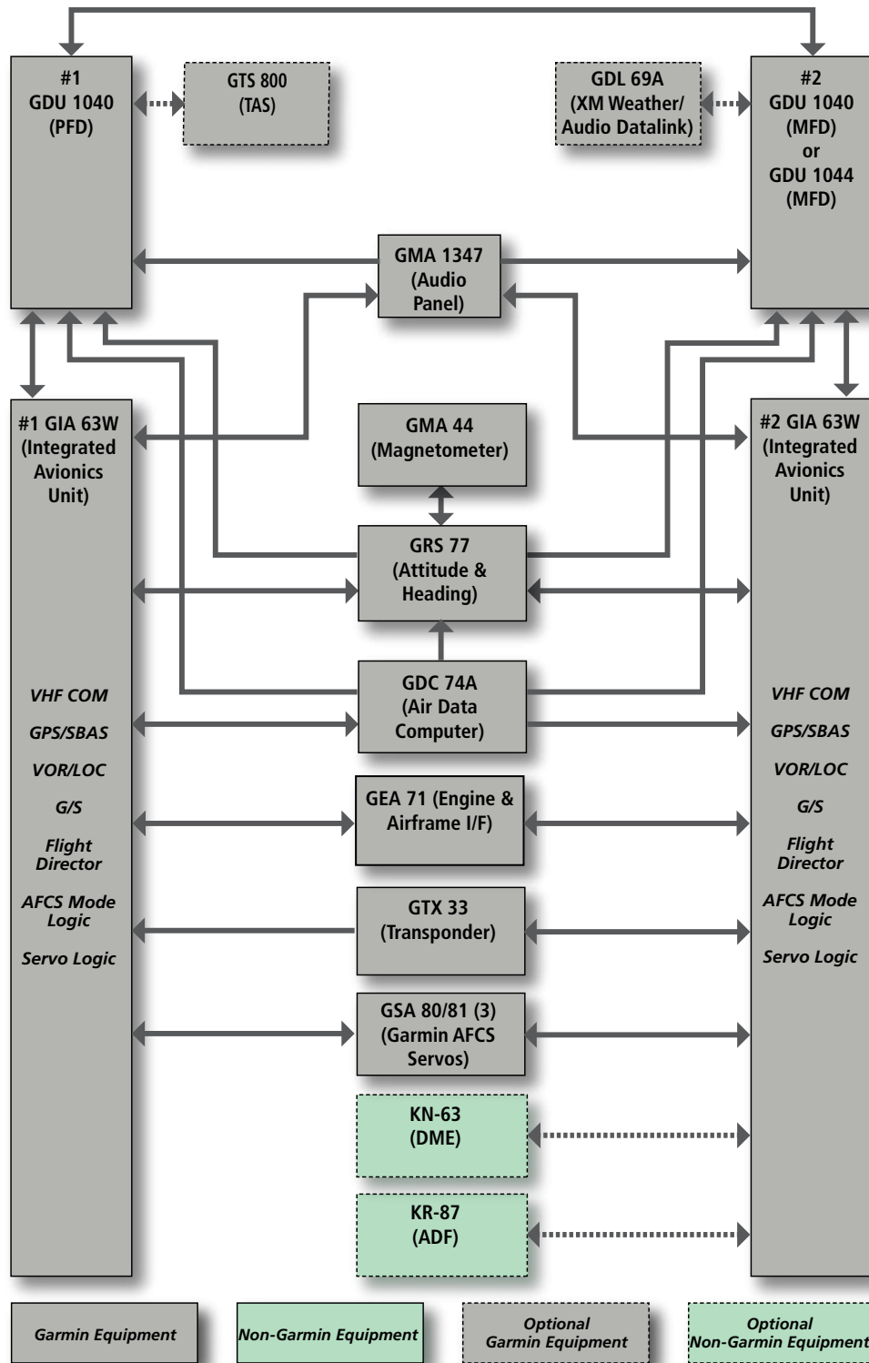
Figure 1-1 System Block Diagram
