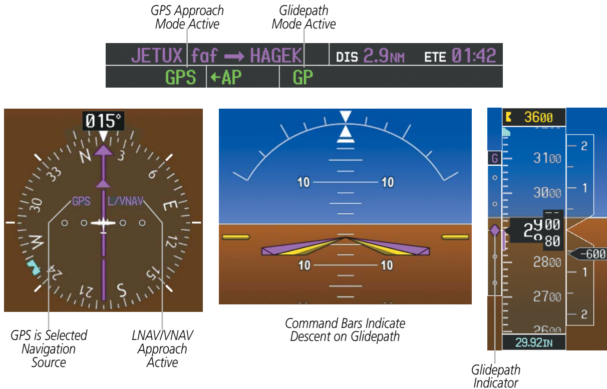
Figure 7-16 Glidepath Mode
