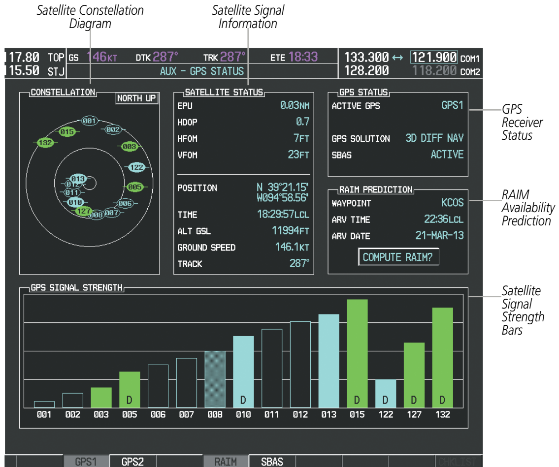
Figure 1-10 GPS Status Page
