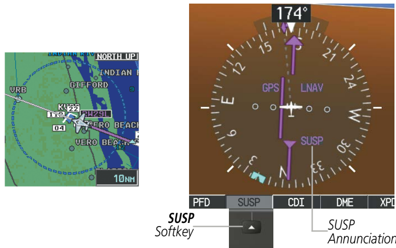
Figure 2-28 Suspending Automatic Waypoint Sequencing
